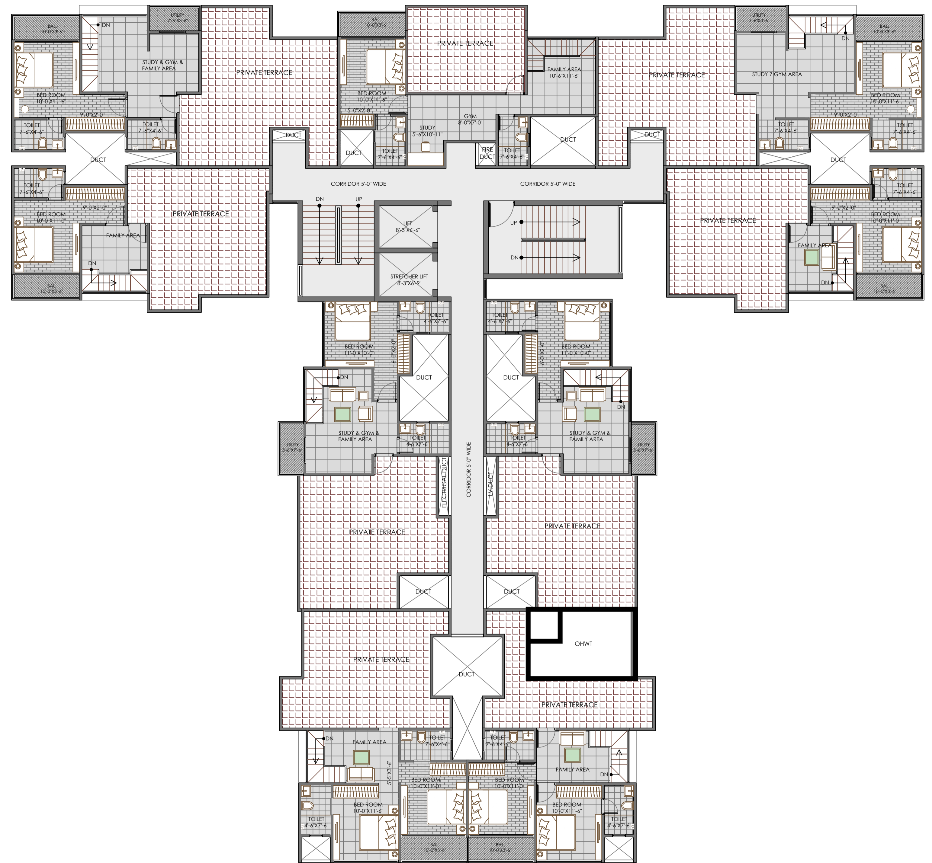
TOWER C2 - 13th UPPER FLOOR PLAN
