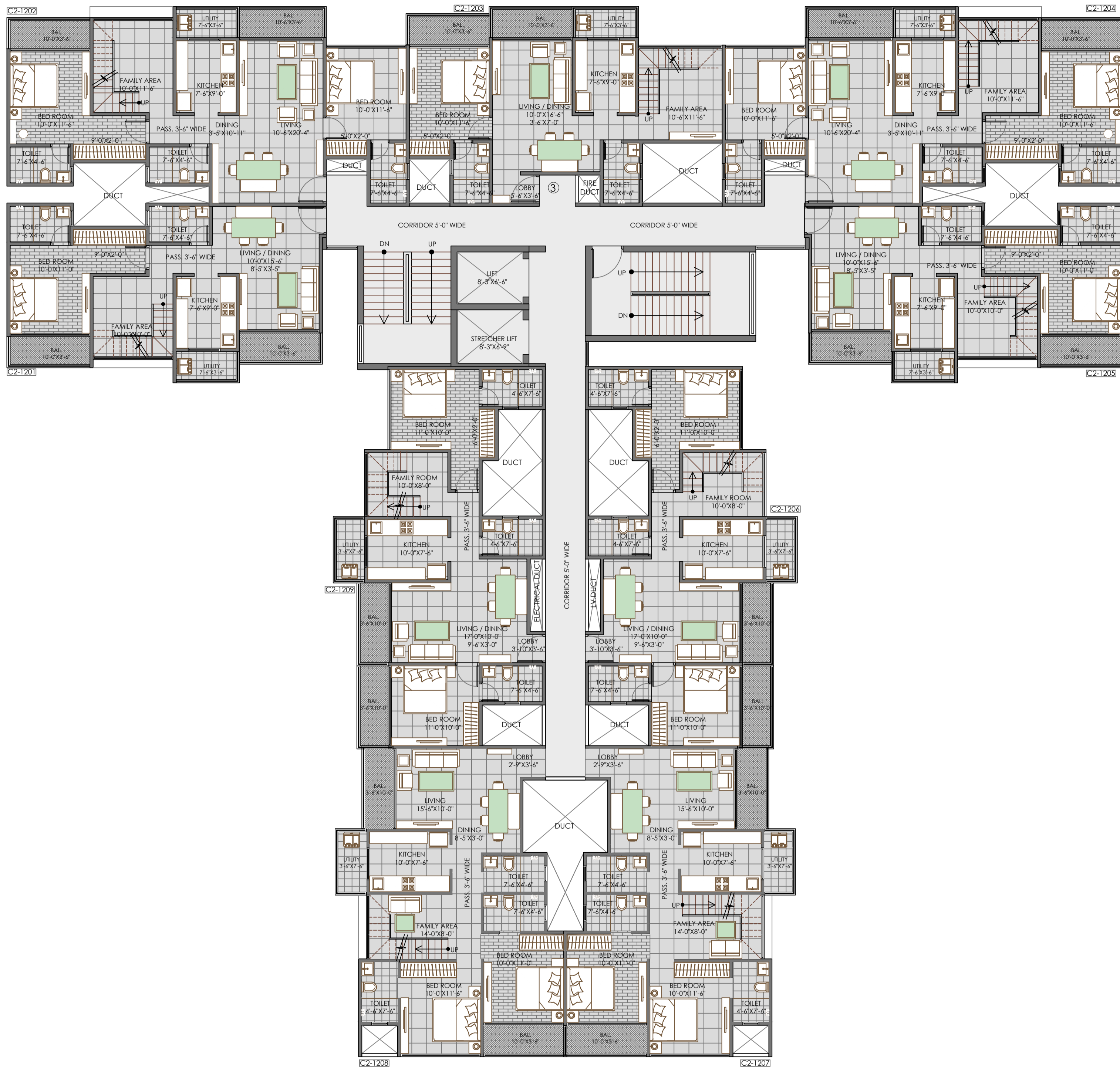
TOWER C2 - 12th LOWER FLOOR PLAN
